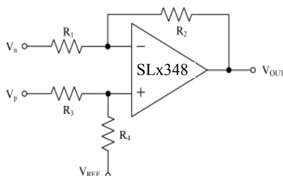
Figure 14 Differential Amplifier
