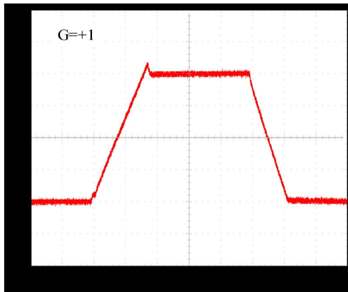
Figure 8 Large-Signal Step Response at 5V
