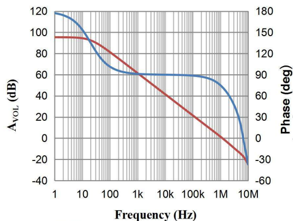
Figure 2 Open-loop Gain and Phase as a function of Frequency
