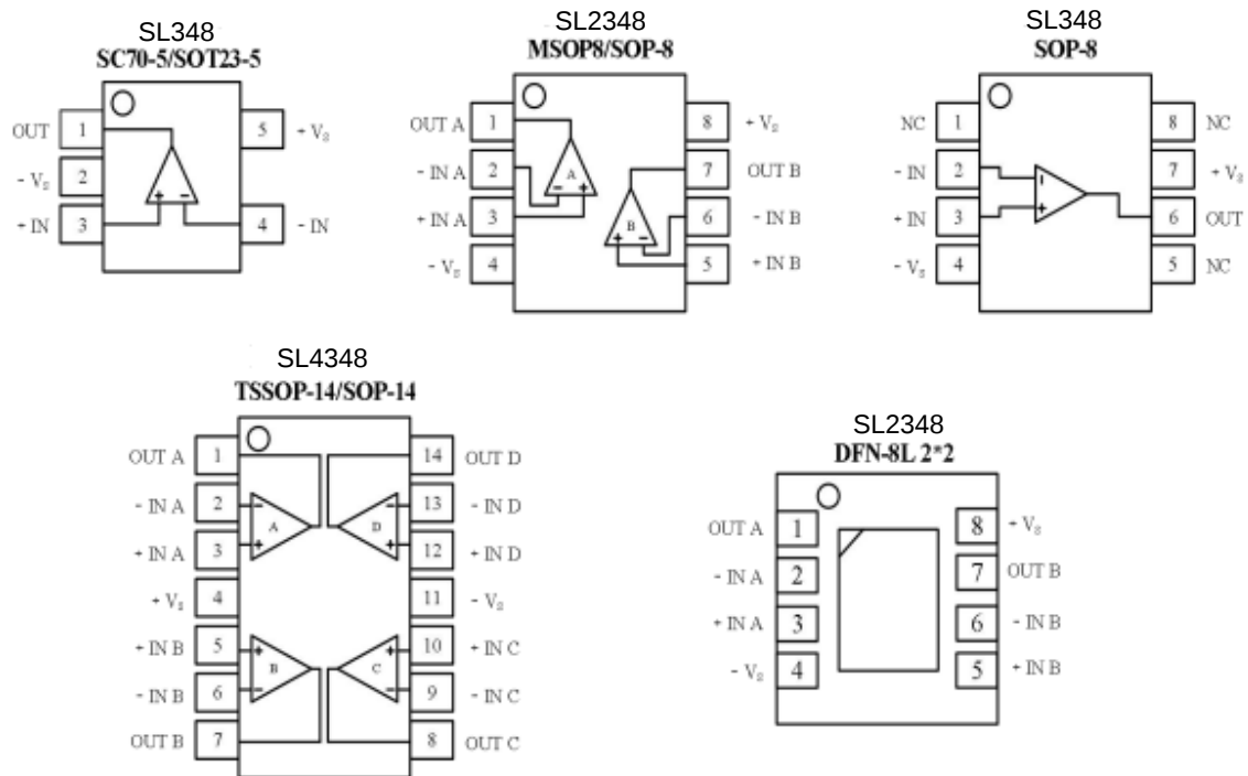
Figure 1 Pin Configurations
