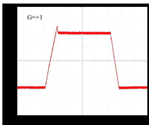
Figure 6 Large-Signal Step Response at 2.7V
